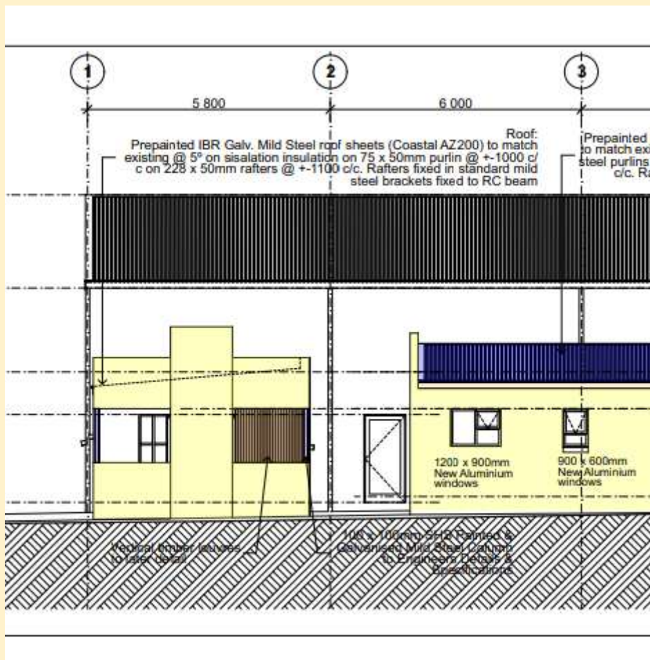
East Elevation
