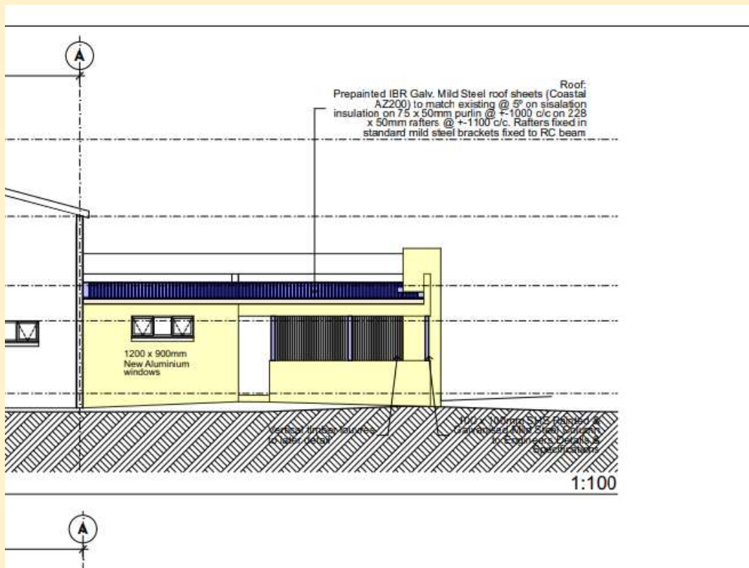
East Elevation
