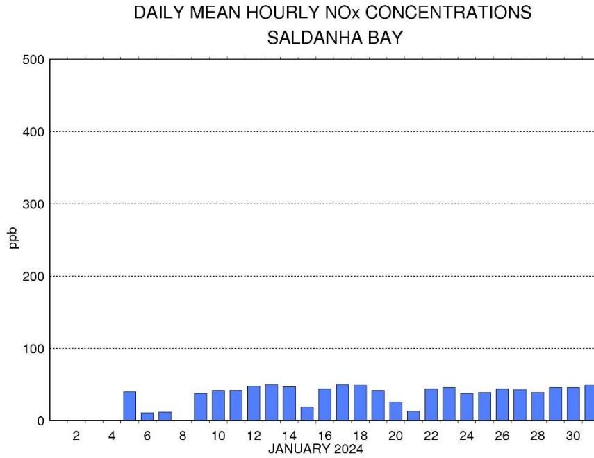
Figure 4.1-4 Daily Mean Hourly NO x Concentrations at Saldanha Bay in January 2024
