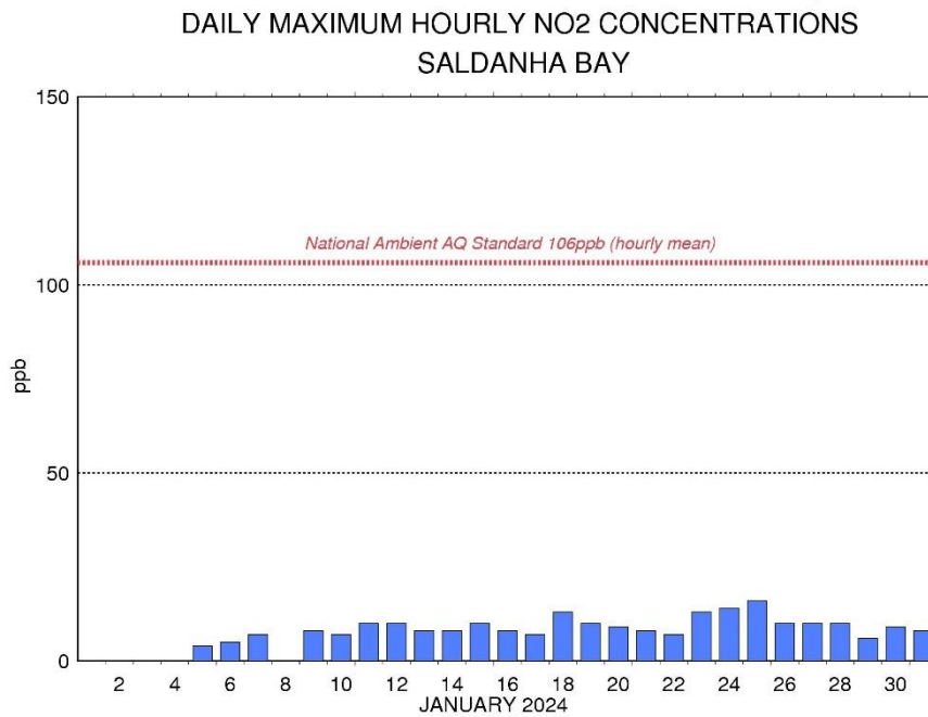
Figure 4.1-3 Daily Maximum NO 2 Concentrations at Saldanha Bay in January 2024
