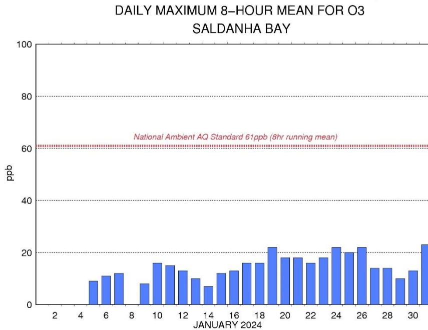
Figure 4.1-5 Daily Maximum Eight-hourly O 3 Concentrations at Saldanha Bay in January 2024
