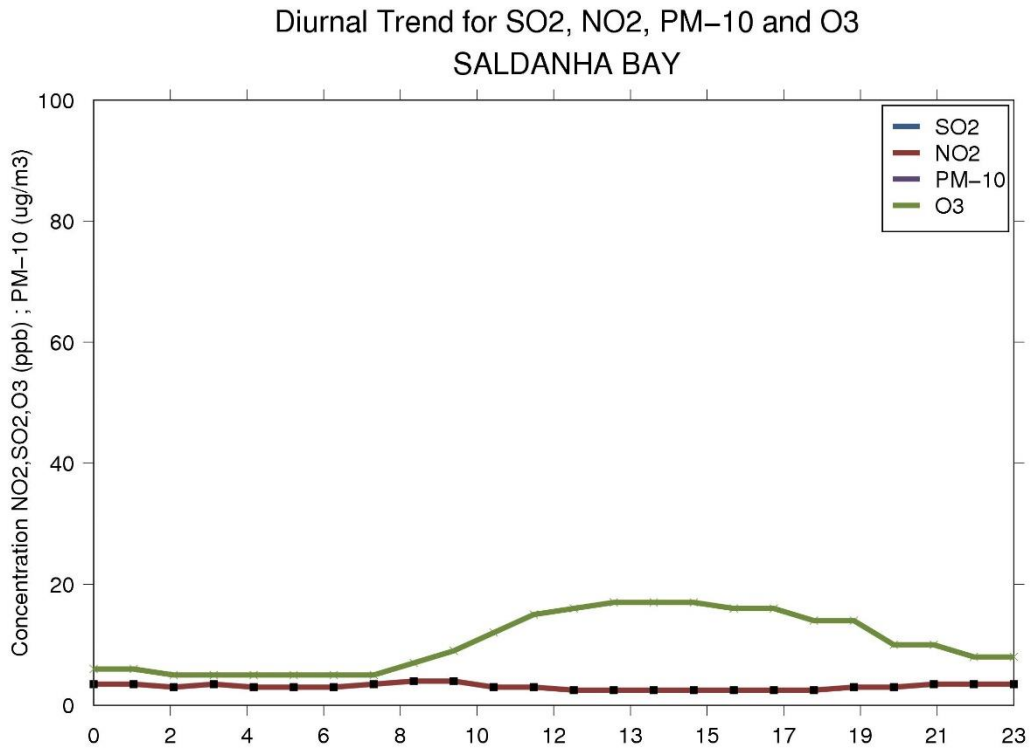
Figure 4.4-1 Diurnal Trend for Ambient Air Pollutants at Saldanha Bay in January 2024
