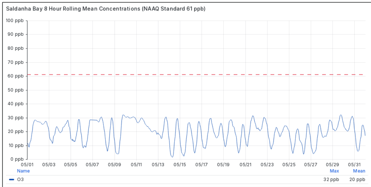
Figure 4.1-5 Eight-hourly Rolling Mean O 3 Concentrations at Saldanha Bay in May 2026
