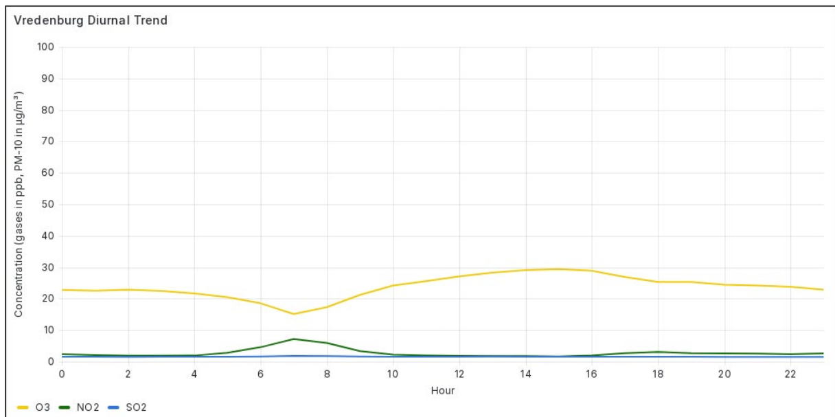
Figure 4.5-2 Diurnal Trend for Ambient Air Pollutants at Vredenburg in May 2026
