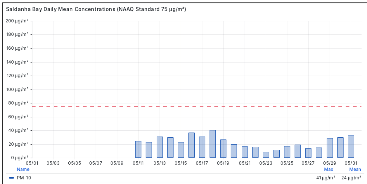
Figure 4.1-6 Daily Mean PM-10 Concentrations at Saldanha Bay in May 2026
