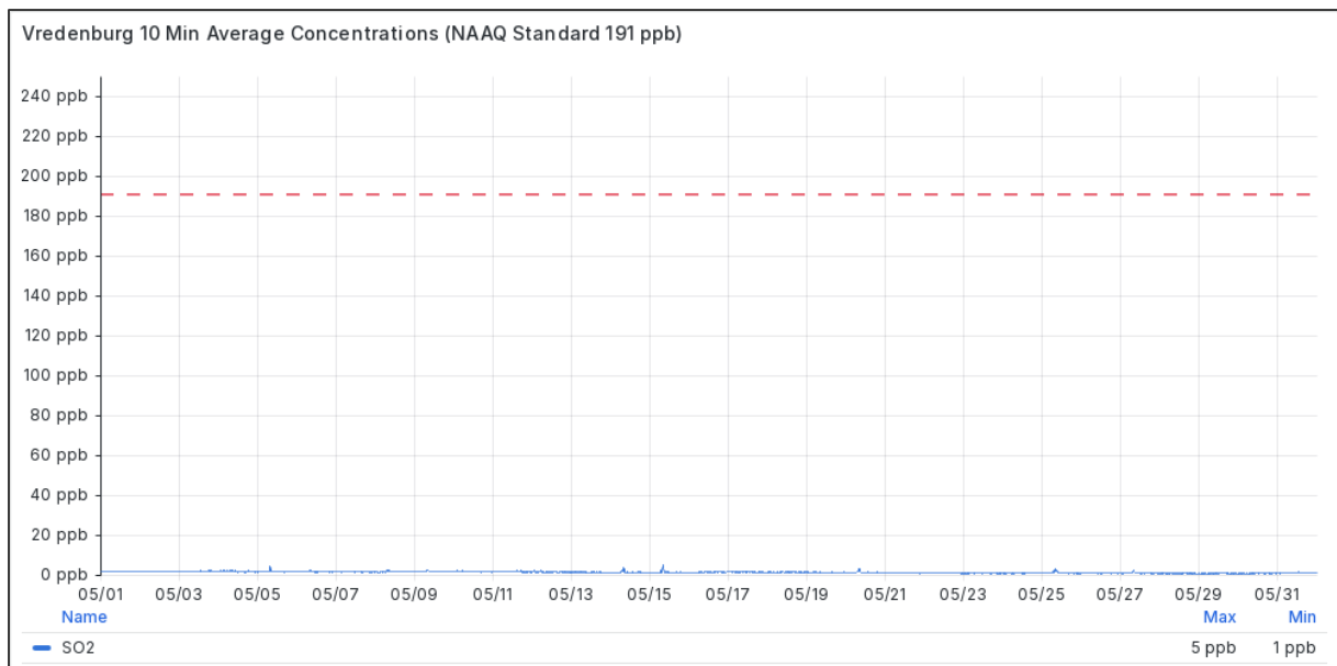
Figure 4.2-2 Daily Maximum 10-minute SO 2 Concentrations at Vredenburg in May 2026
