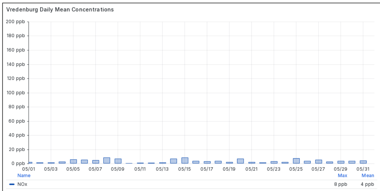
Figure 4.2-4 Daily Mean Hourly NO x Concentrations at Vredenburg in May 2026
