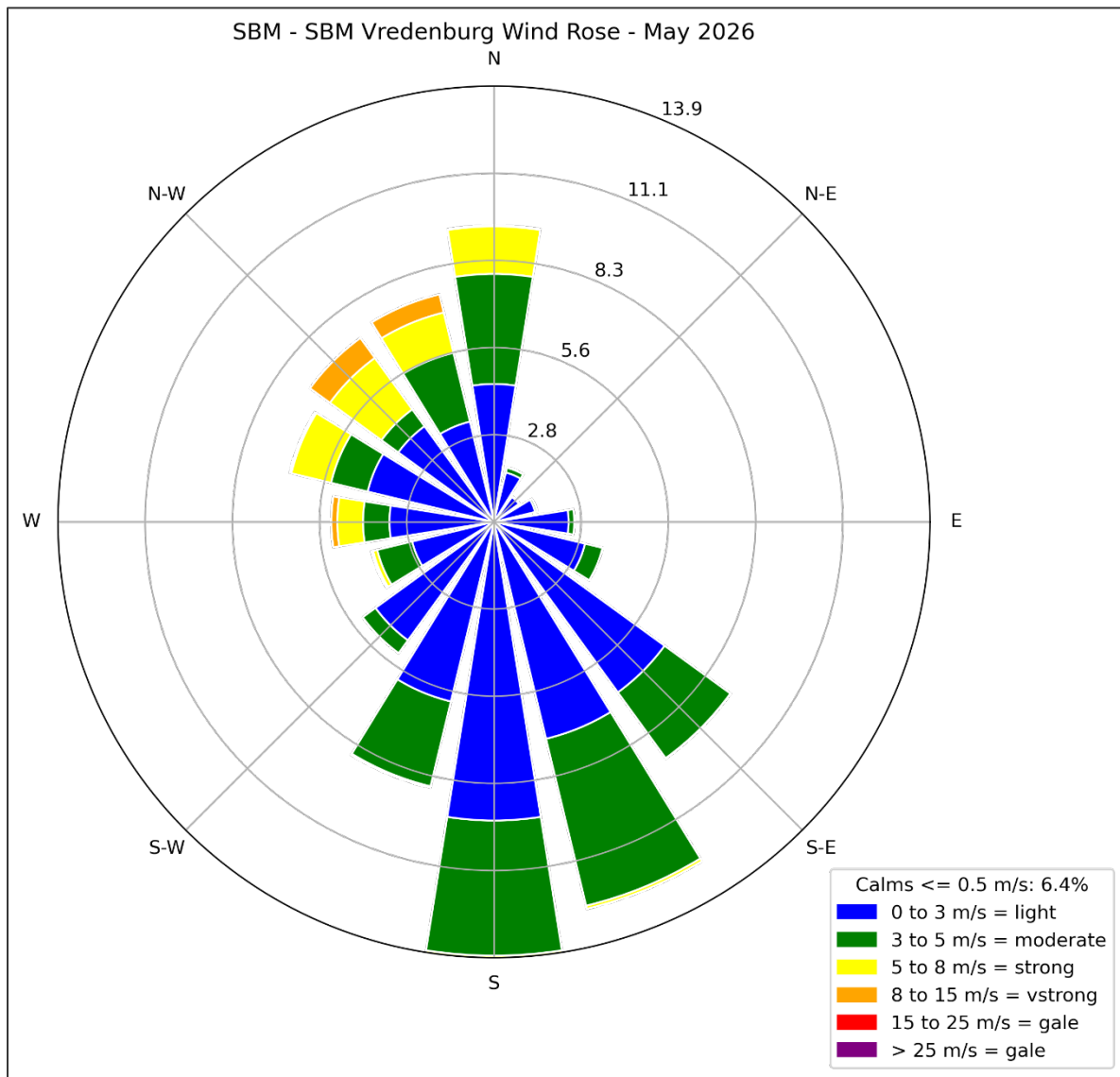
Figure 4.6-2 Wind Rose for Vredenburg for May 2026
