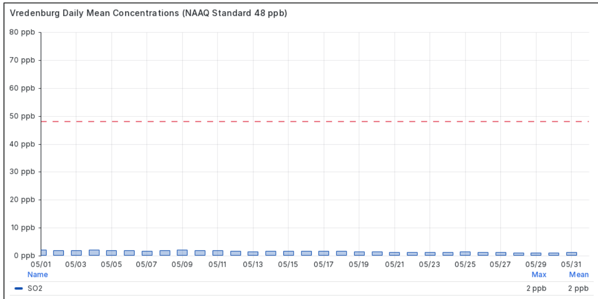
Figure 4.2-1 Daily Mean Hourly SO 2 Concentrations at Vredenburg in May 2026
