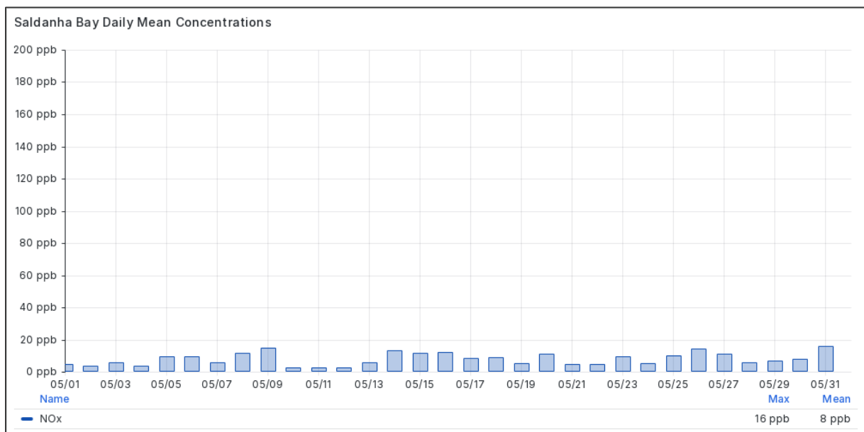
Figure 4.1-4 Daily Mean NO x Concentrations at Saldanha Bay in May 2026
