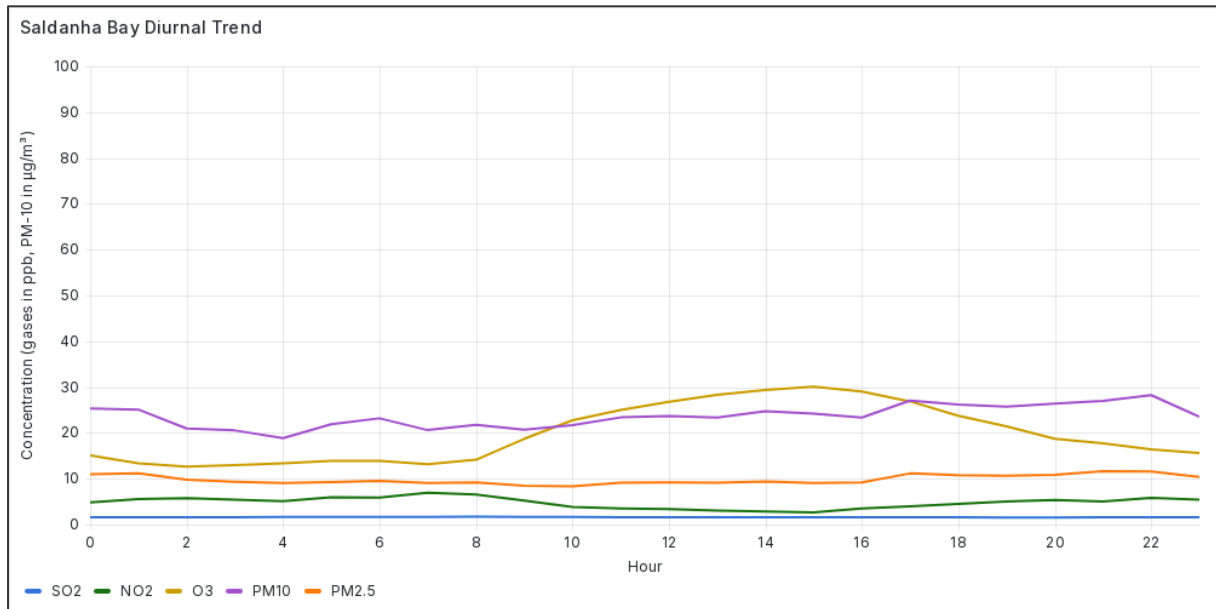
Figure 4.5-1 Diurnal Trend for Ambient Air Pollutants at Saldanha Bay in May 2026
