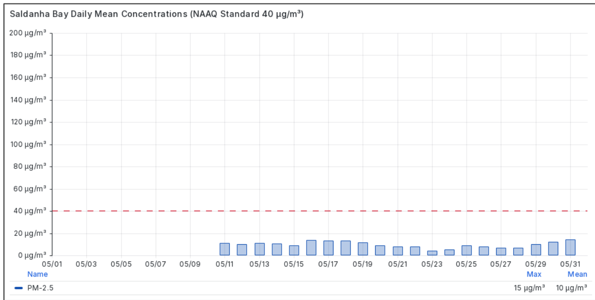
Figure 4.1-7 Daily Mean PM-2.5 Concentrations at Saldanha Bay in May 2026
