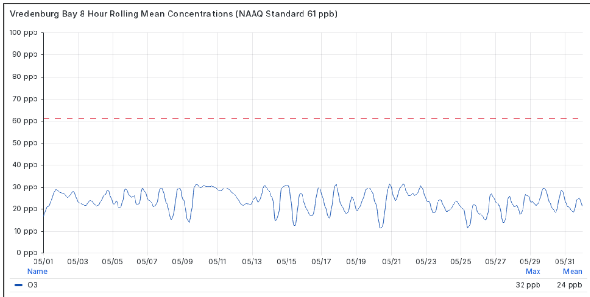
Figure 4.2-5 Eight-hourly Rolling Mean O 3 Concentrations at Vredenburg in May 2026
