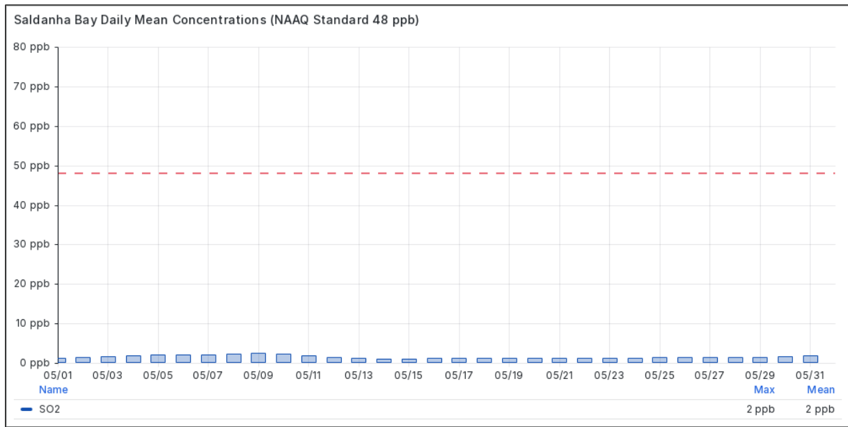
Figure 4.1-1 Daily Mean SO 2 Concentrations at Saldanha Bay in May 2026
