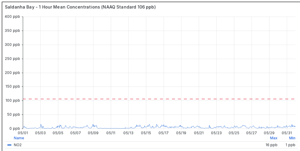
Figure 4.1-3 1 Hourly Mean NO 2 Concentrations at Saldanha Bay in May 2026
