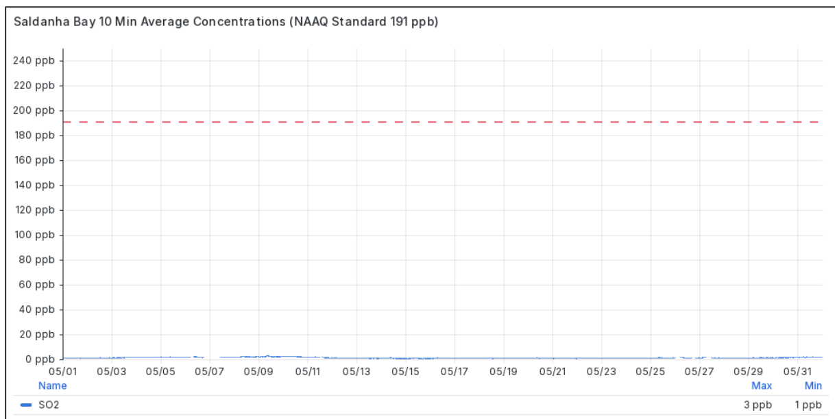
Figure 4.1-2 Mean 10-minute SO 2 Concentrations at Saldanha Bay in May 2026
