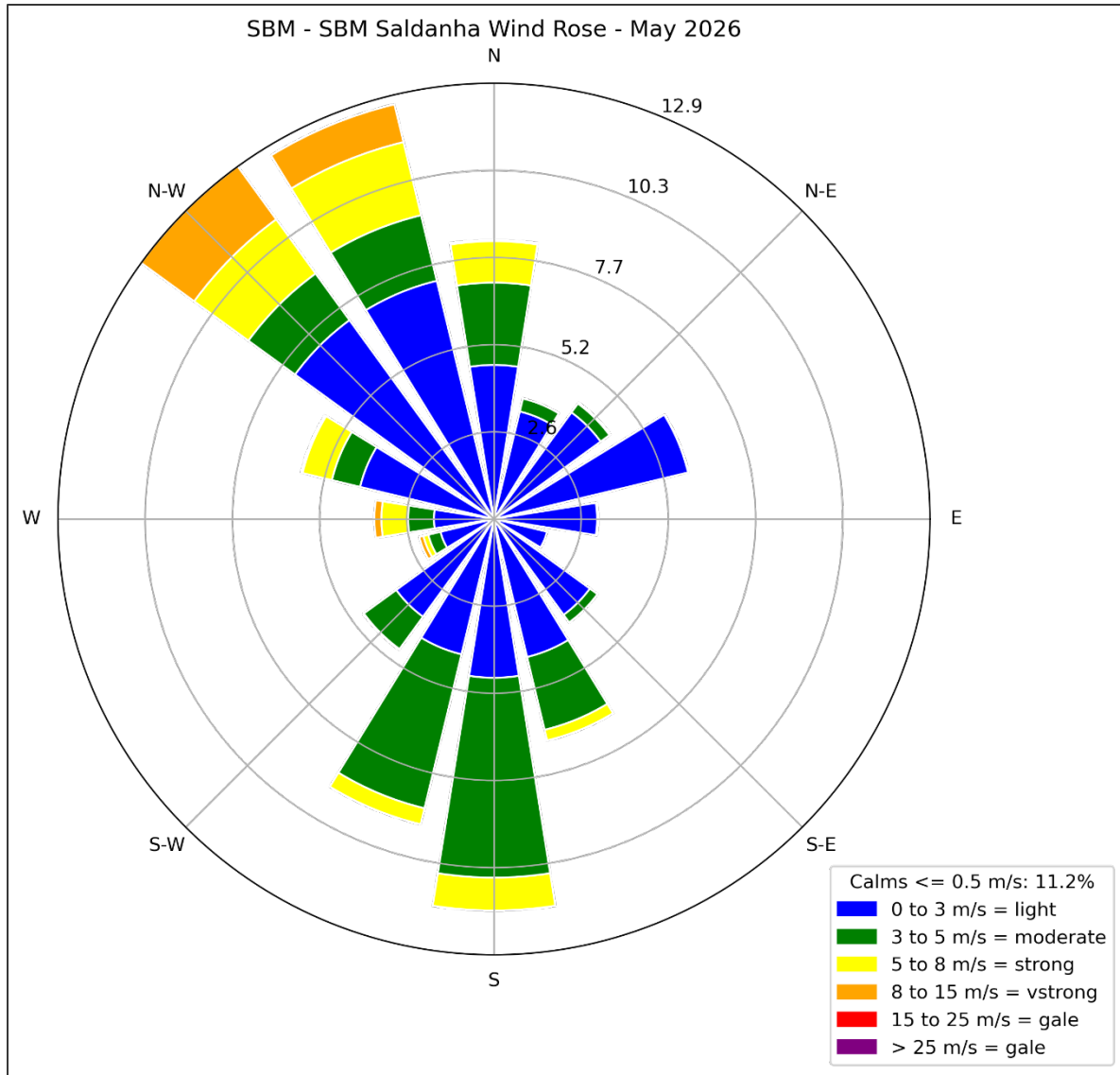
Figure 4.6-1 Wind Rose for Saldanha Bay for May 2026
