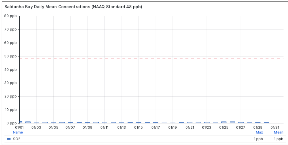
Figure 4.1-1 Daily Mean SO 2 Concentrations at Saldanha Bay in January 2026
