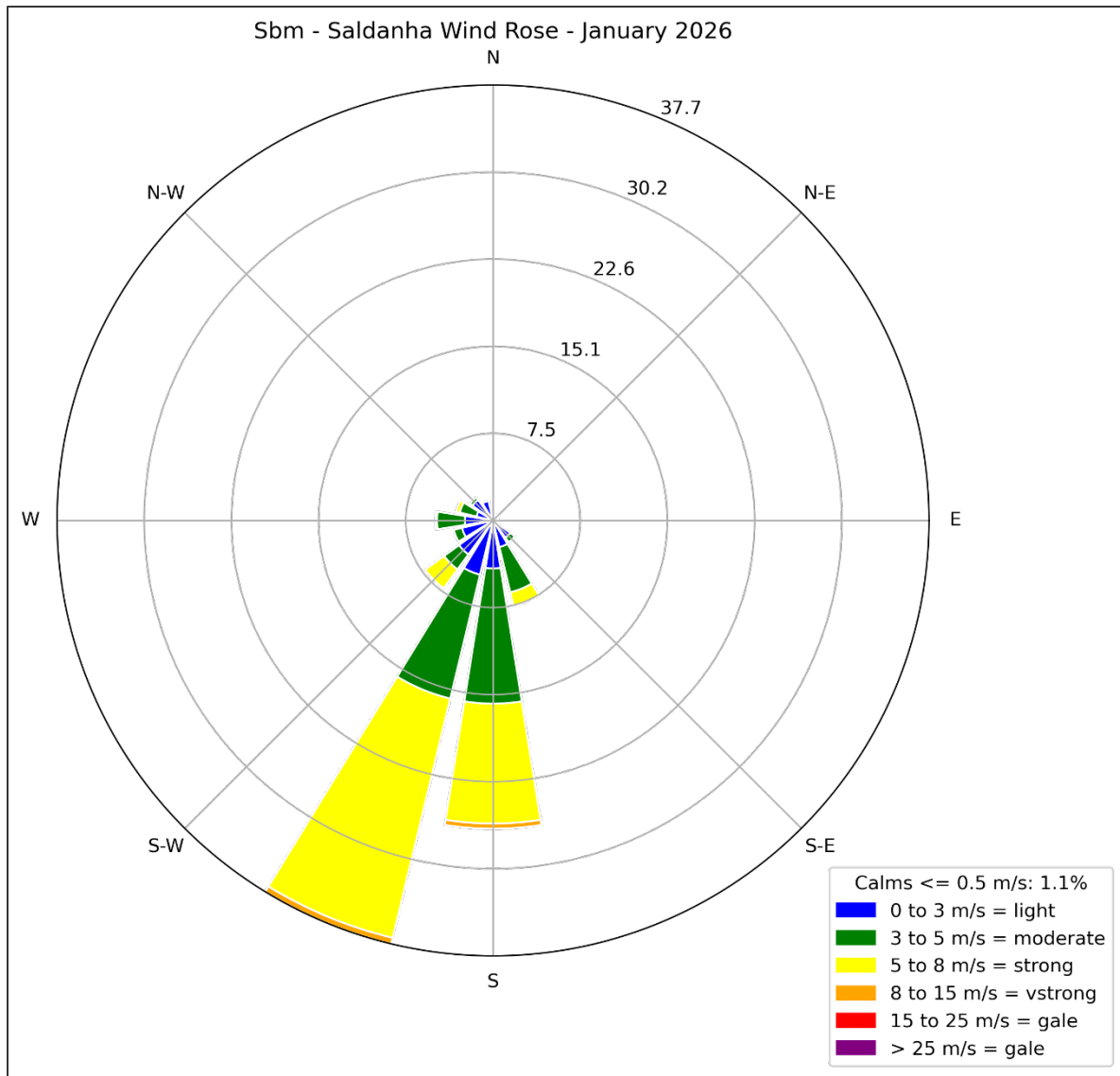
Figure 4.6-1 Wind Rose for Saldanha Bay for January 2026
