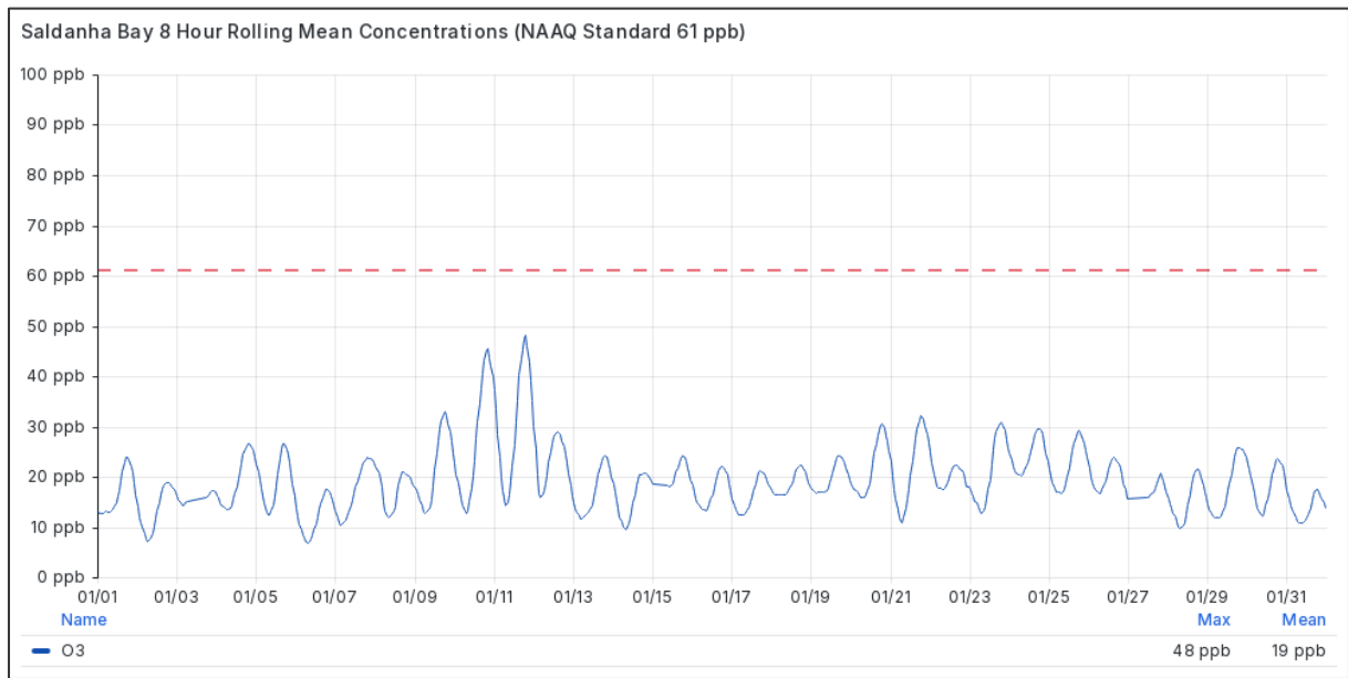
Figure 4.1-5 Eight-hourly Rolling Mean O 3 Concentrations at Saldanha Bay in January 2026
