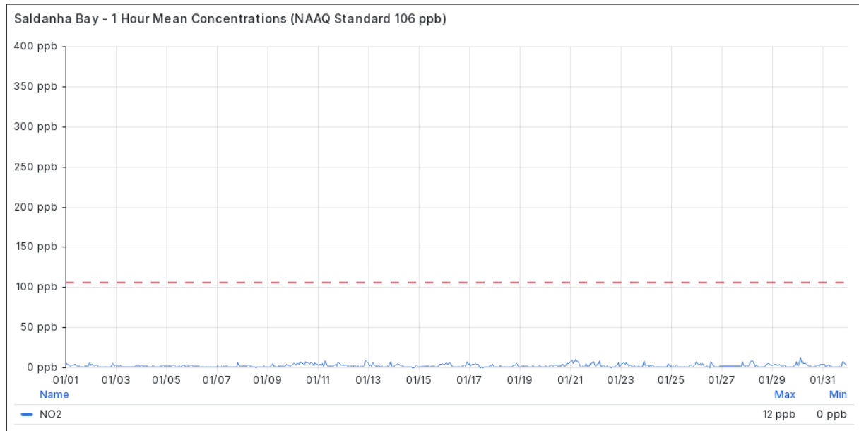
Figure 4.1-3 1 Hourly Mean NO 2 Concentrations at Saldanha Bay in January 2026
