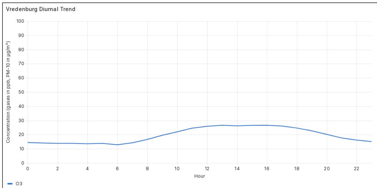
Figure 4.5-2 Diurnal Trend for Ambient Air Pollutants at Vredenburg in January 2026
