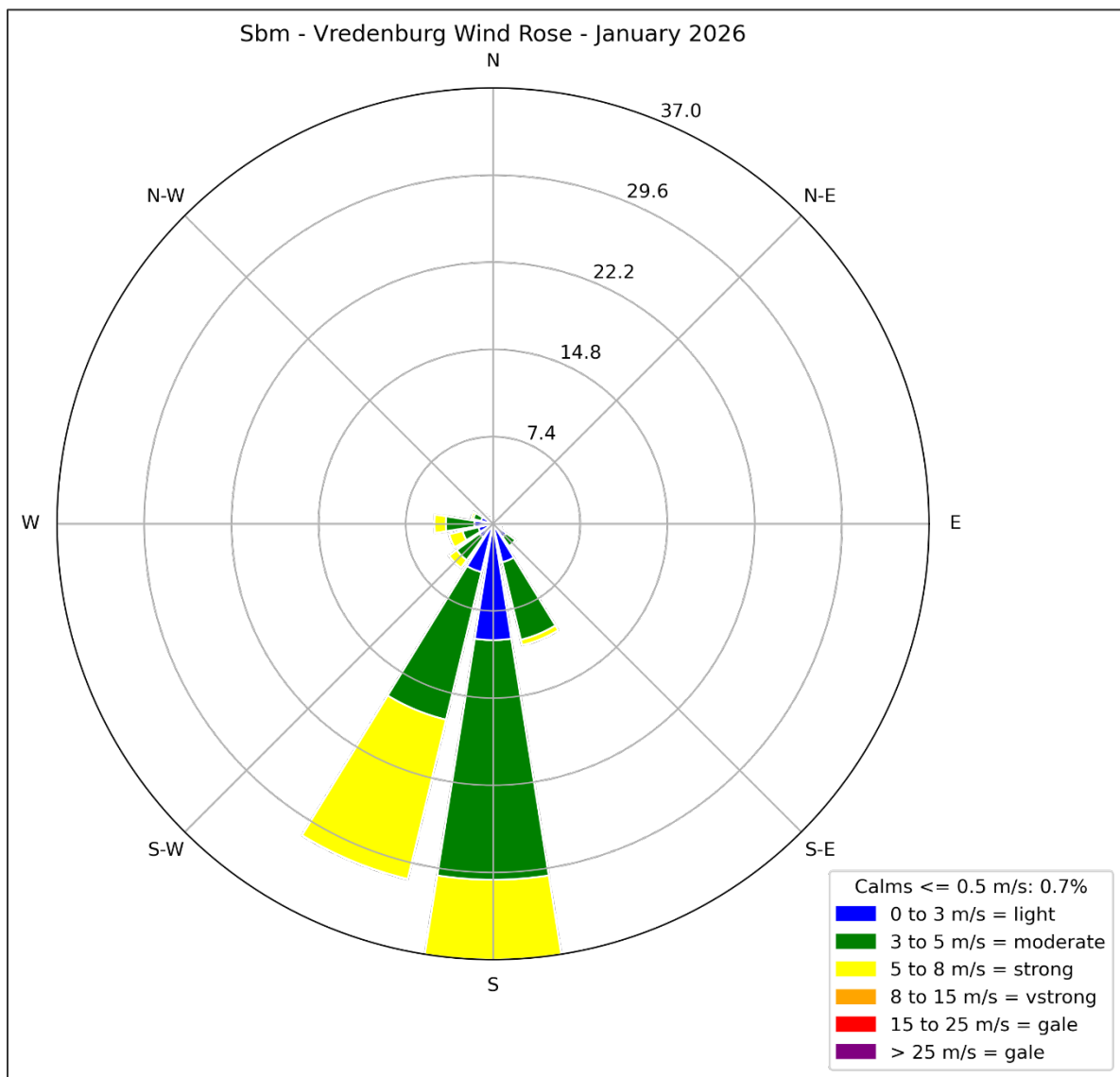
Figure 4.6-2 Wind Rose for Vredenburg for January 2026
