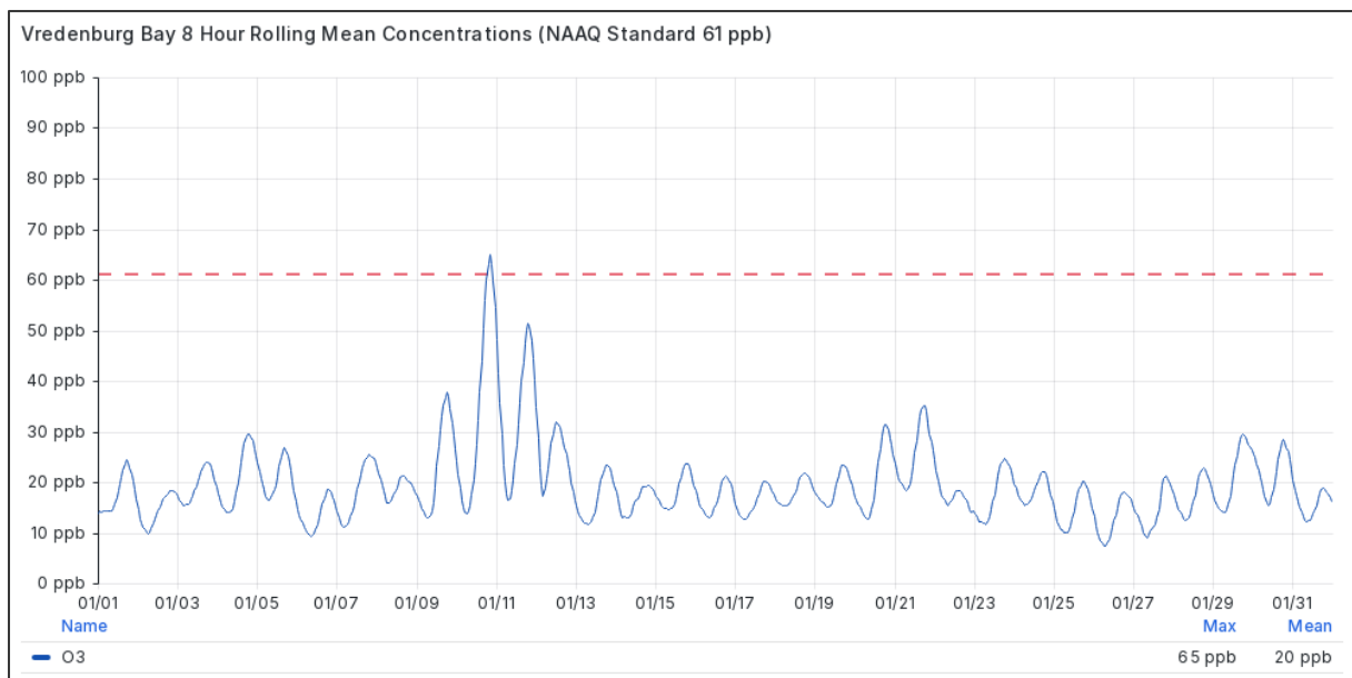
Figure 4.2-5 Eight-hourly Rolling Mean O 3 Concentrations at Vredenburg in January 2026
