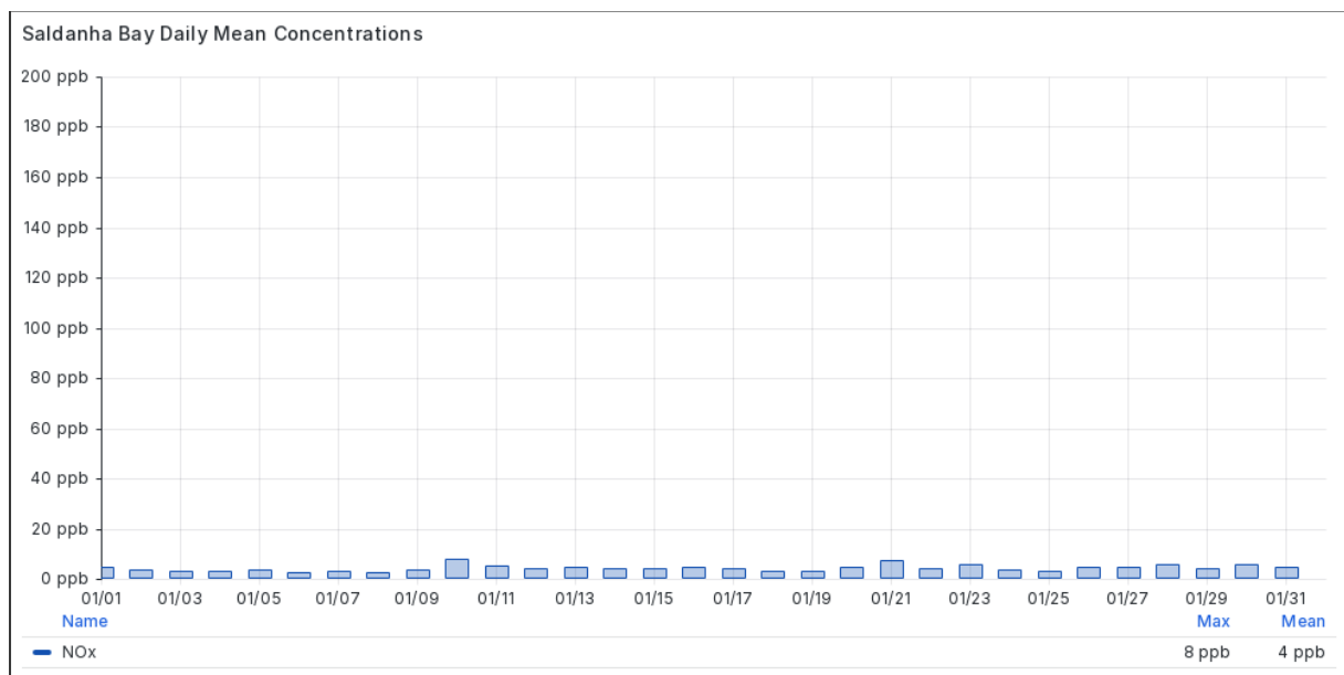
Figure 4.1-4 Daily Mean NO x Concentrations at Saldanha Bay in January 2026
