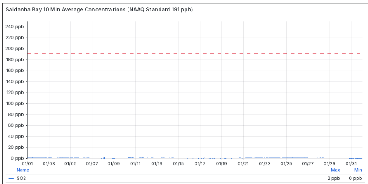
Figure 4.1-2 Mean 10-minute SO 2 Concentrations at Saldanha Bay in January 2026
