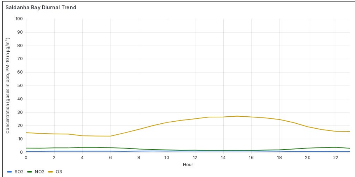
Figure 4.5-1 Diurnal Trend for Ambient Air Pollutants at Saldanha Bay in January 2026
