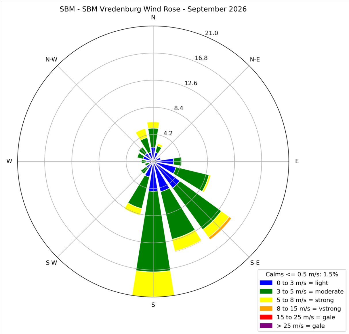
Figure 4.6-2 Wind Rose for Vredenburg for September 2026
