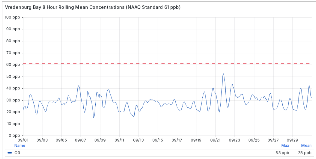
Figure 4.2-5 Eight-hourly Rolling Mean O 3 Concentrations at Vredenburg in September 2026
