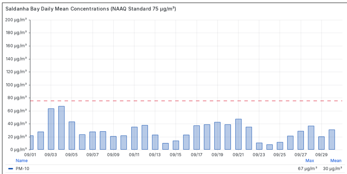
Figure 4.1-6 Daily Mean PM-10 Concentrations at Saldanha Bay in September 2026
