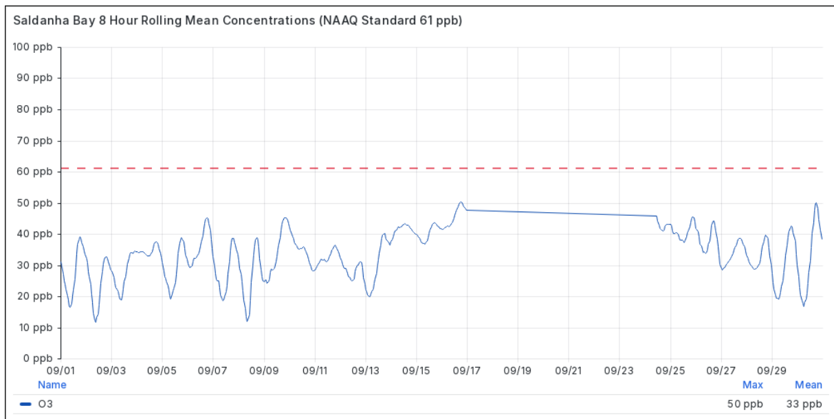
Figure 4.1-5 Eight-hourly Rolling Mean O 3 Concentrations at Saldanha Bay in September 2026
