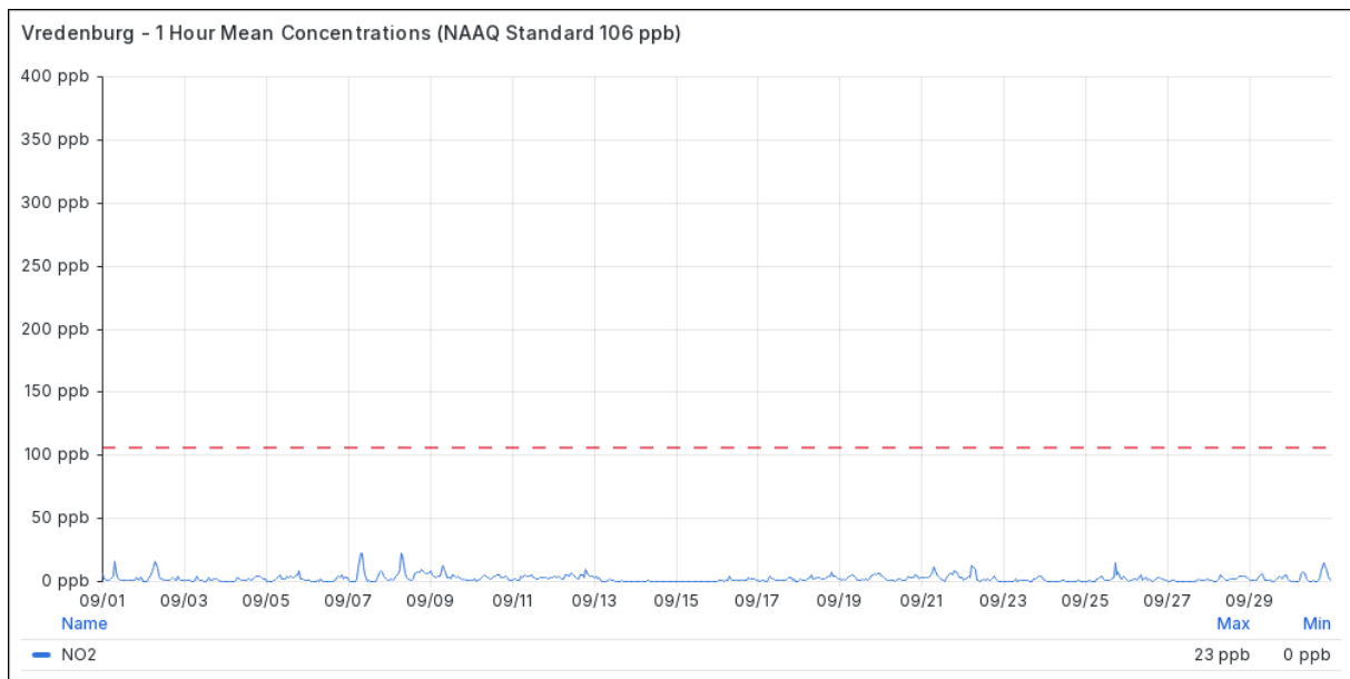
Figure 4.2-3 Daily Maximum NO 2 Concentrations at Vredenburg in September 2026
