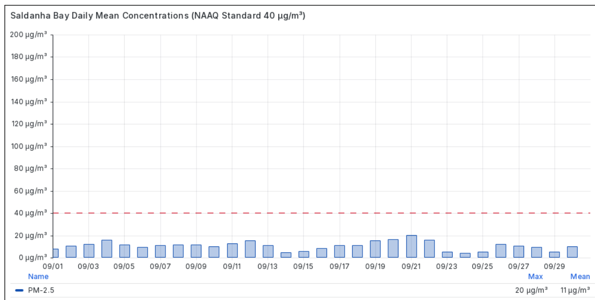
Figure 4.1-7 Daily Mean PM-2.5 Concentrations at Saldanha Bay in September 2026
