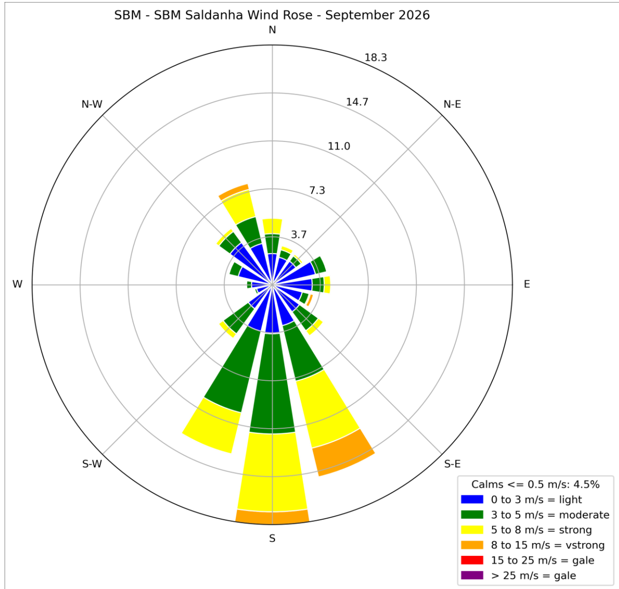
Figure 4.6-1 Wind Rose for Saldanha Bay for September 2026
