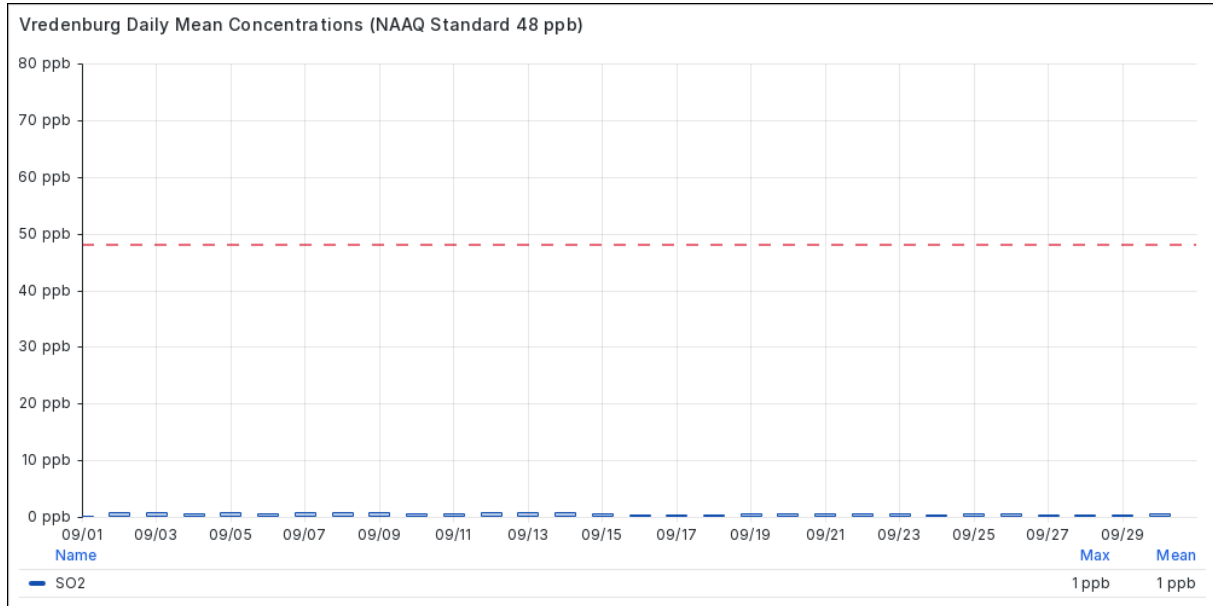
Figure 4.2-1 Daily Mean Hourly SO 2 Concentrations at Vredenburg in September 2026
