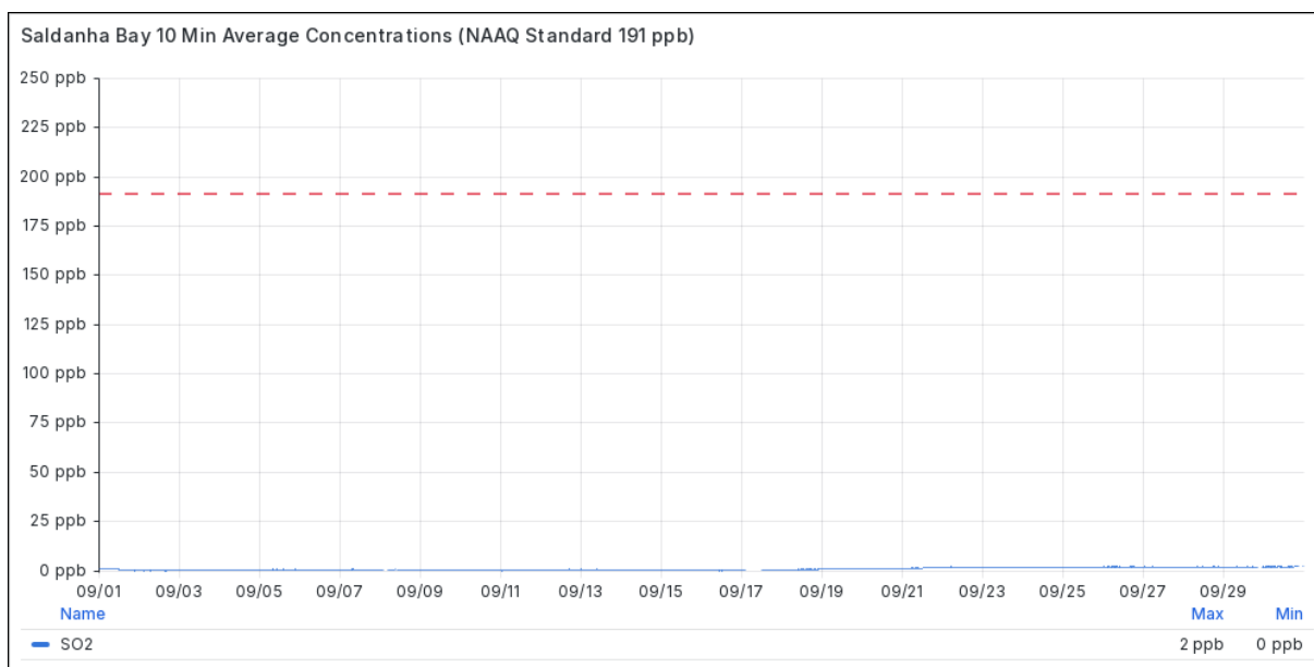
Figure 4.1-2 Mean 10-minute SO 2 Concentrations at Saldanha Bay in September 2026
