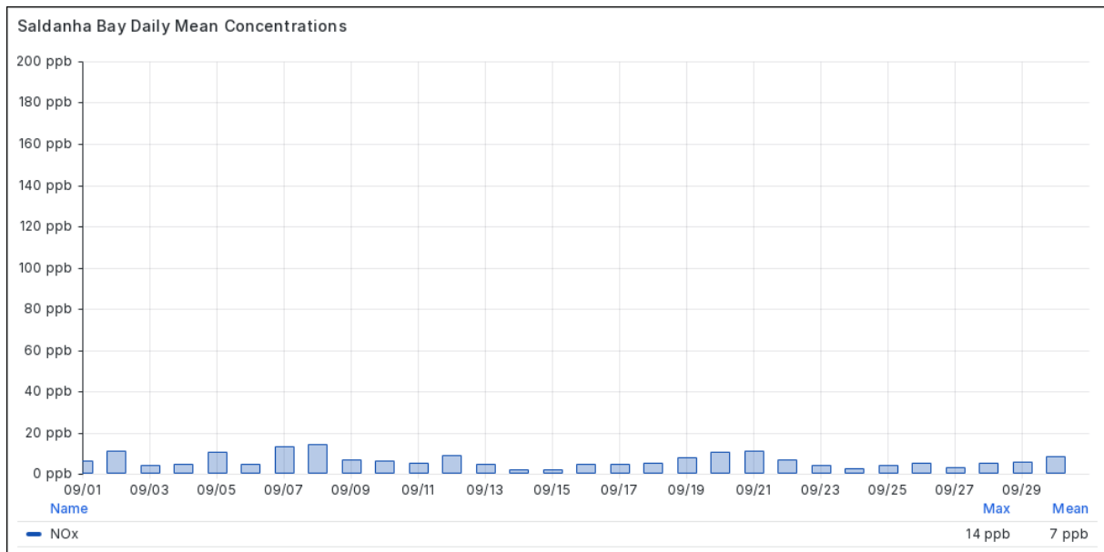
Figure 4.1-4 Daily Mean NO x Concentrations at Saldanha Bay in September 2026
