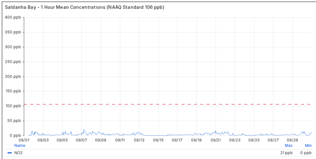
Figure 4.1-3 1 Hourly Mean NO 2 Concentrations at Saldanha Bay in September 2026
