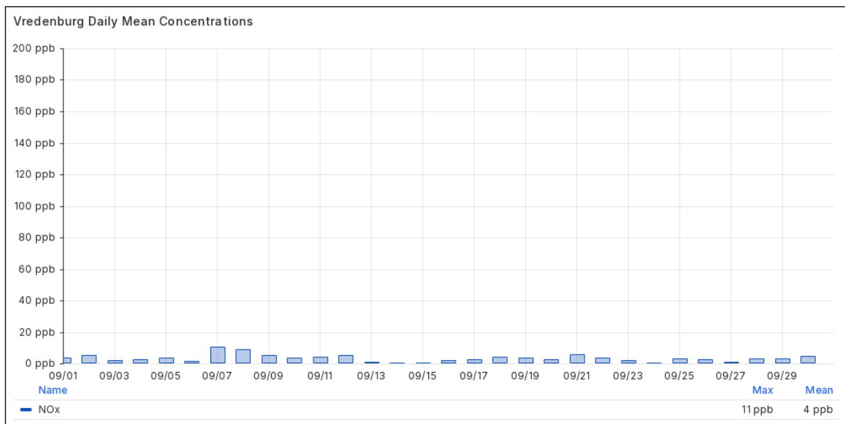
Figure 4.2-4 Daily Mean Hourly NO x Concentrations at Vredenburg in September 2026
