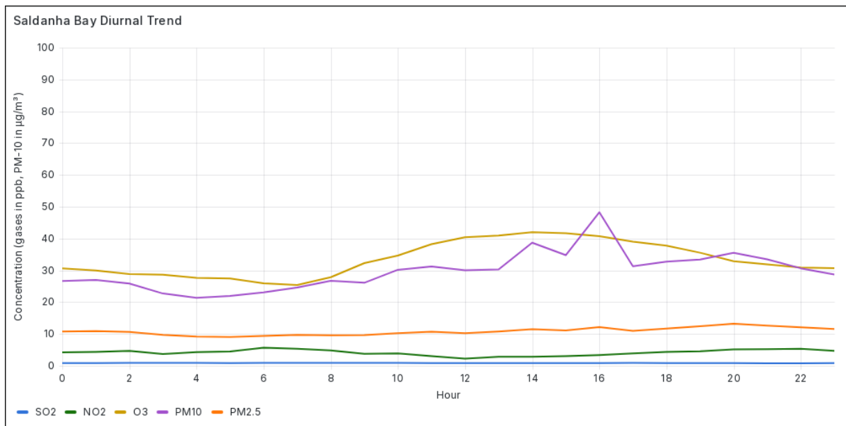
Figure 4.5.1 Diurnal Trend for Ambient Air Pollutants at Saldanha Bay in September 2026
