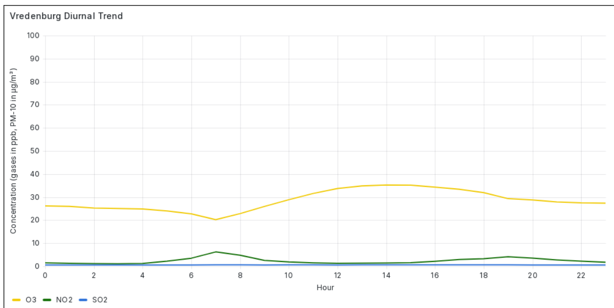
Figure 4.5-2 Diurnal Trend for Ambient Air Pollutants at Vredenburg in September 2026
