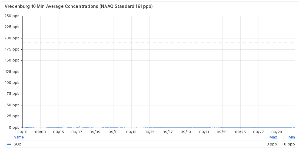
Figure 4.2-2 Daily Maximum 10-minute SO 2 Concentrations at Vredenburg in September 2026
