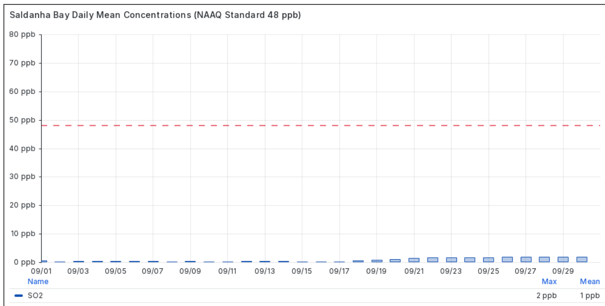
Figure 4.1-1 Daily Mean SO 2 Concentrations at Saldanha Bay in September 2026
