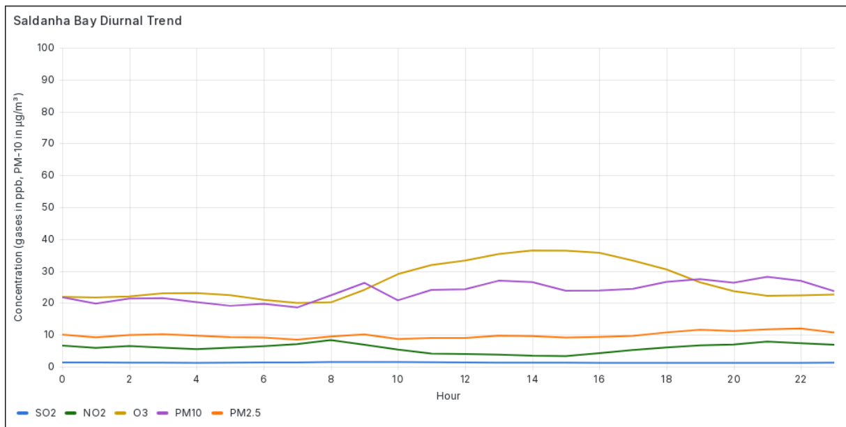
Figure 4.5.1 Diurnal Trend for Ambient Air Pollutants at Saldanha Bay in June 2026
