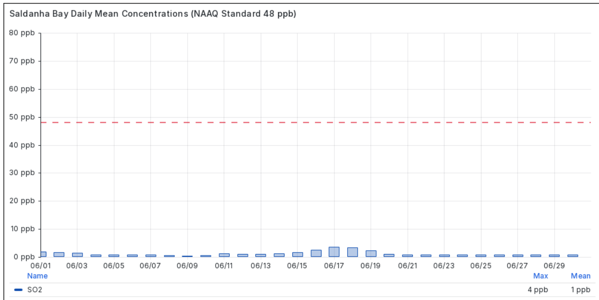
Figure 4.1-1 Daily Mean SO 2 Concentrations at Saldanha Bay in June 2026
