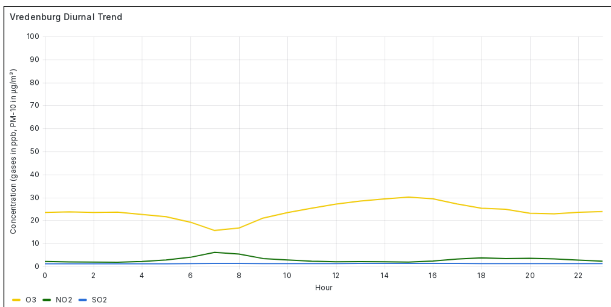
Figure 4.5-2 Diurnal Trend for Ambient Air Pollutants at Vredenburg in June 2026
