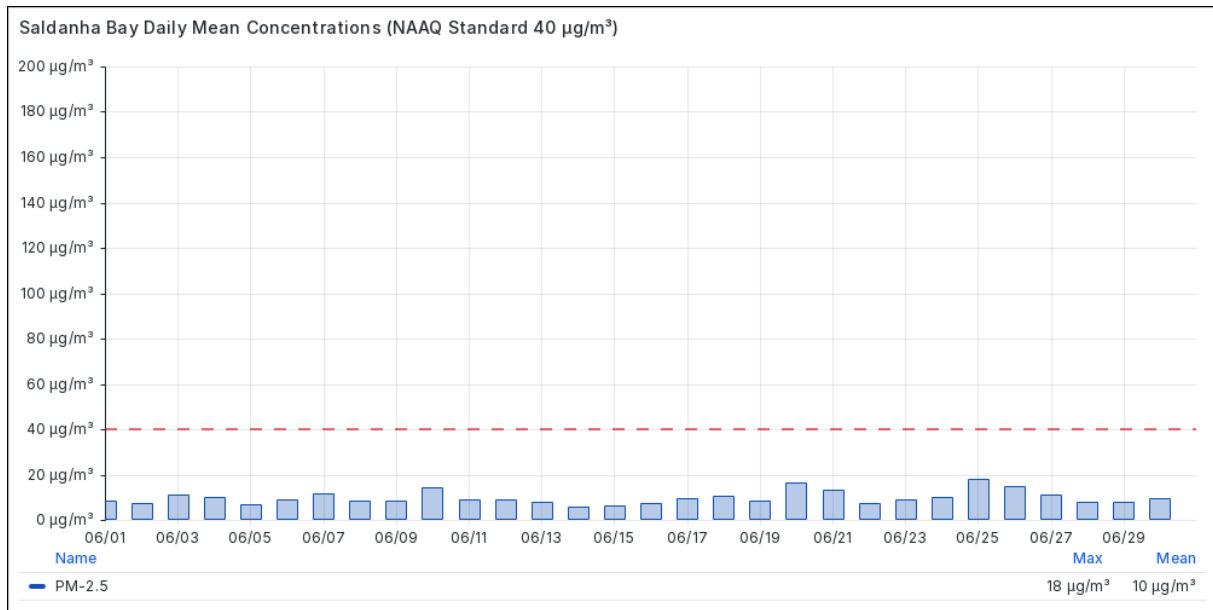
Figure 4.1-7 Daily Mean PM-2.5 Concentrations at Saldanha Bay in June 2026
