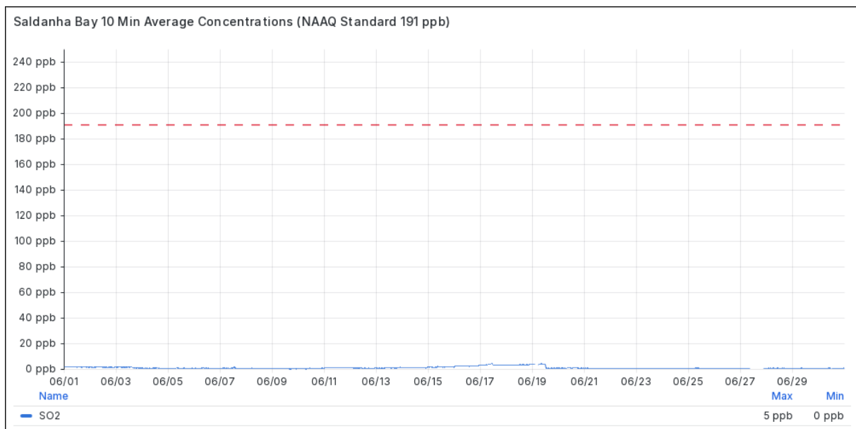
Figure 4.1-2 Mean 10-minute SO 2 Concentrations at Saldanha Bay in June 2026
