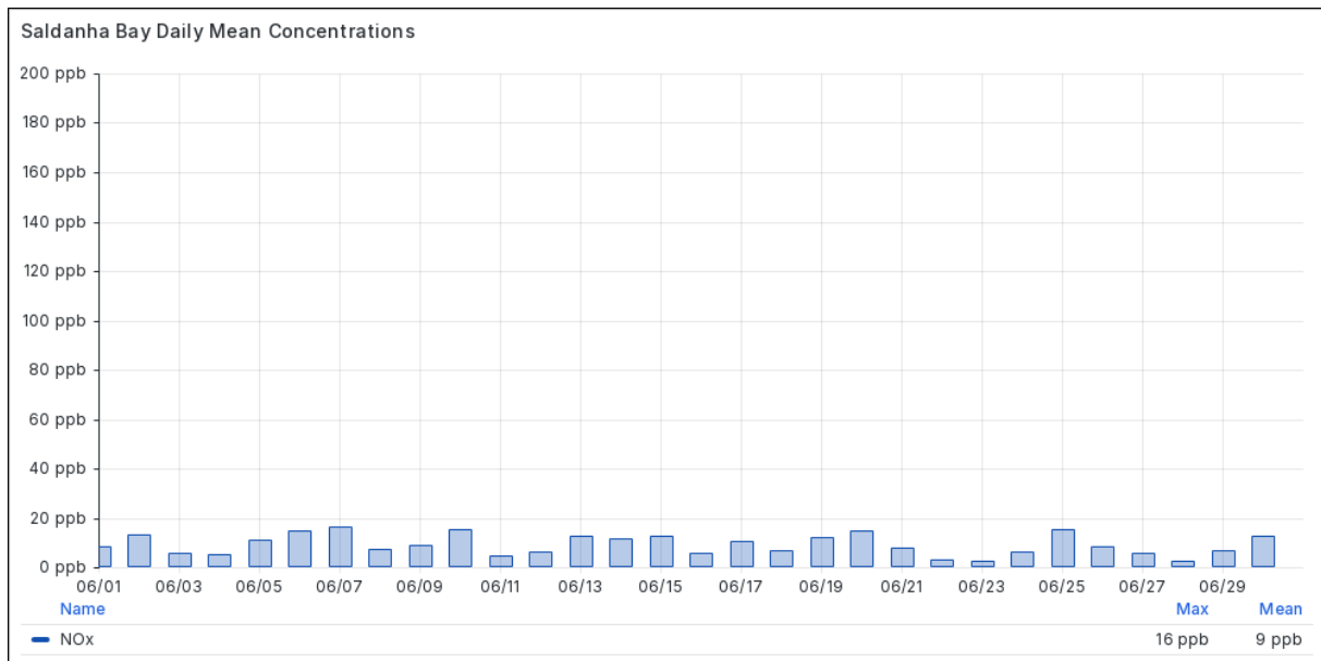
Figure 4.1-4 Daily Mean NO x Concentrations at Saldanha Bay in June 2026
