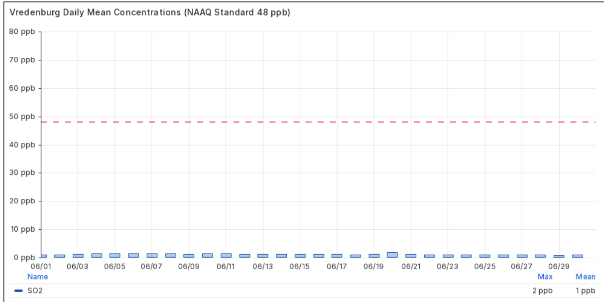
Figure 4.2-1 Daily Mean Hourly SO 2 Concentrations at Vredenburg in June 2026
