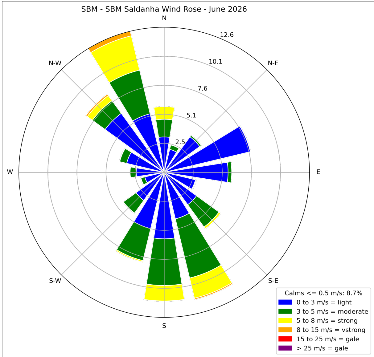
Figure 4.6-1 Wind Rose for Saldanha Bay for June 2026
