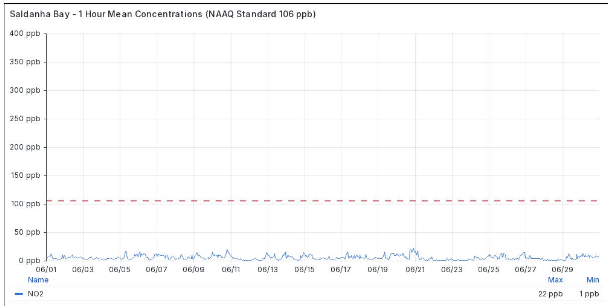
Figure 4.1-3 1 Hourly Mean NO 2 Concentrations at Saldanha Bay in June 2026
