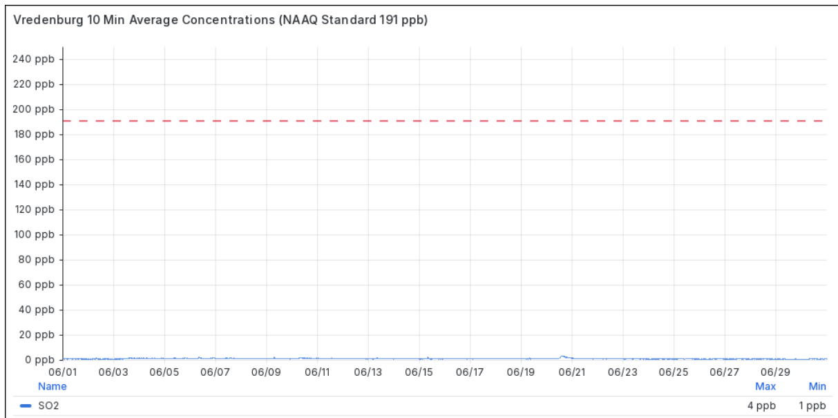
Figure 4.2-2 Daily Maximum 10-minute SO 2 Concentrations at Vredenburg in June 2026
