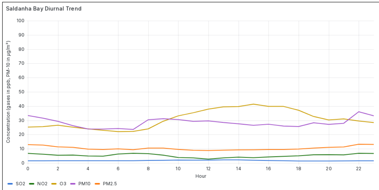
Figure 4.5.1 Diurnal Trend for Ambient Air Pollutants at Saldanha Bay in August 2026
