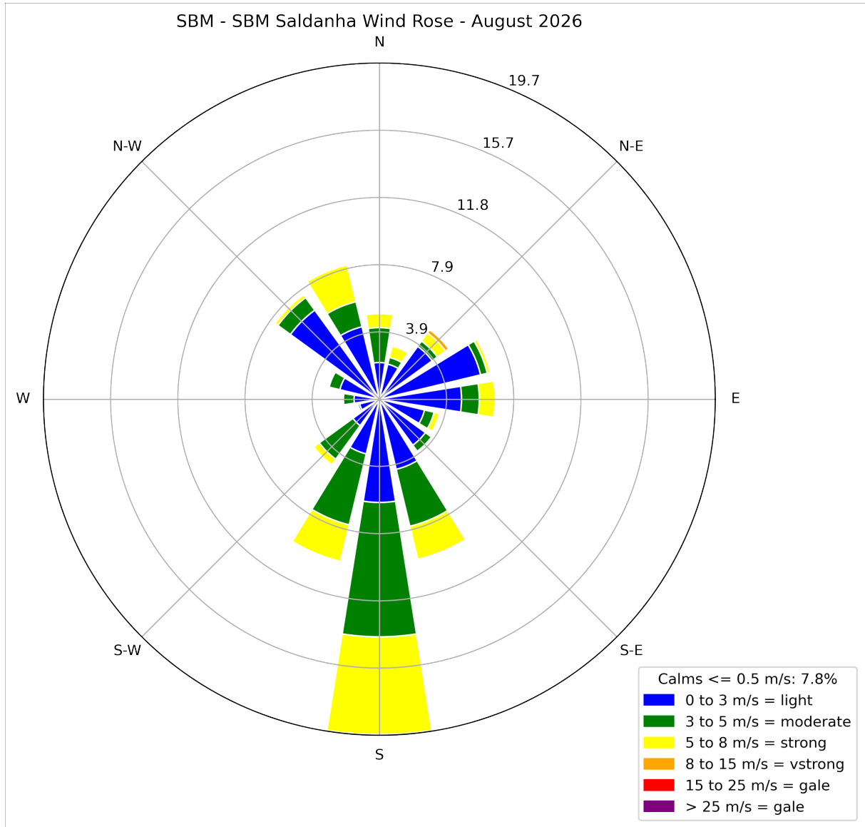
Figure 4.6-1 Wind Rose for Saldanha Bay for August 2026
