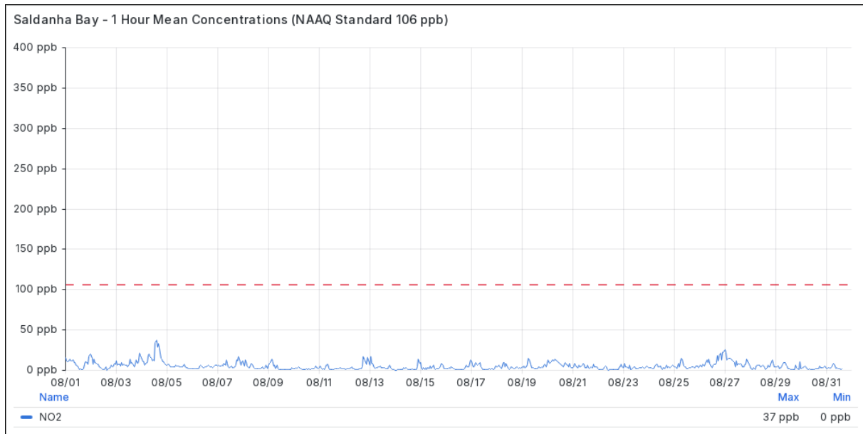
Figure 4.1-3 1 Hourly Mean NO 2 Concentrations at Saldanha Bay in August 2026
