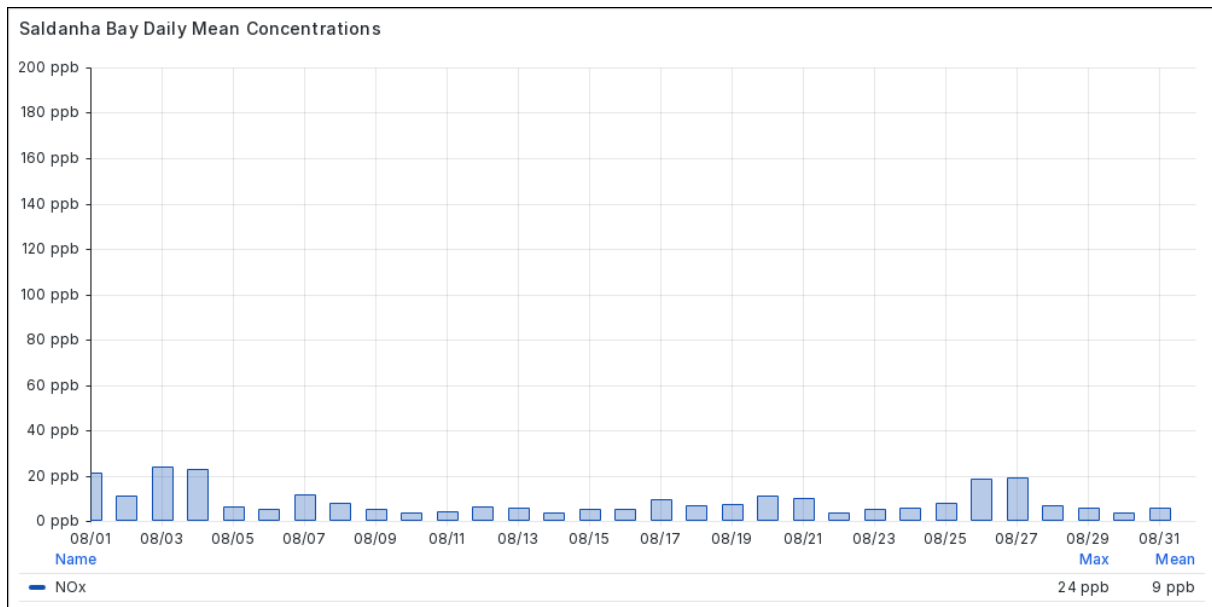
Figure 4.1-4 Daily Mean NO x Concentrations at Saldanha Bay in August 2026
