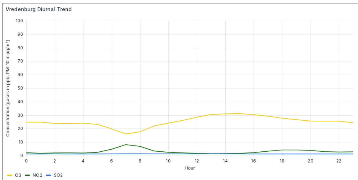
Figure 4.5-2 Diurnal Trend for Ambient Air Pollutants at Vredenburg in August 2026
