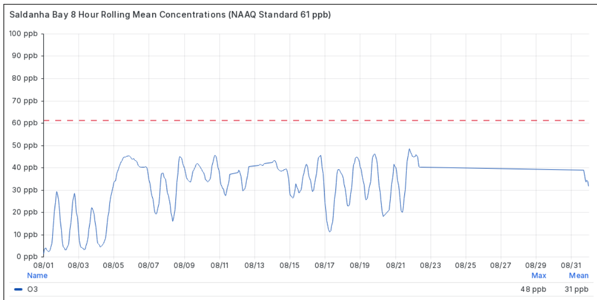
Figure 4.1-5 Eight-hourly Rolling Mean O 3 Concentrations at Saldanha Bay in August 2026
