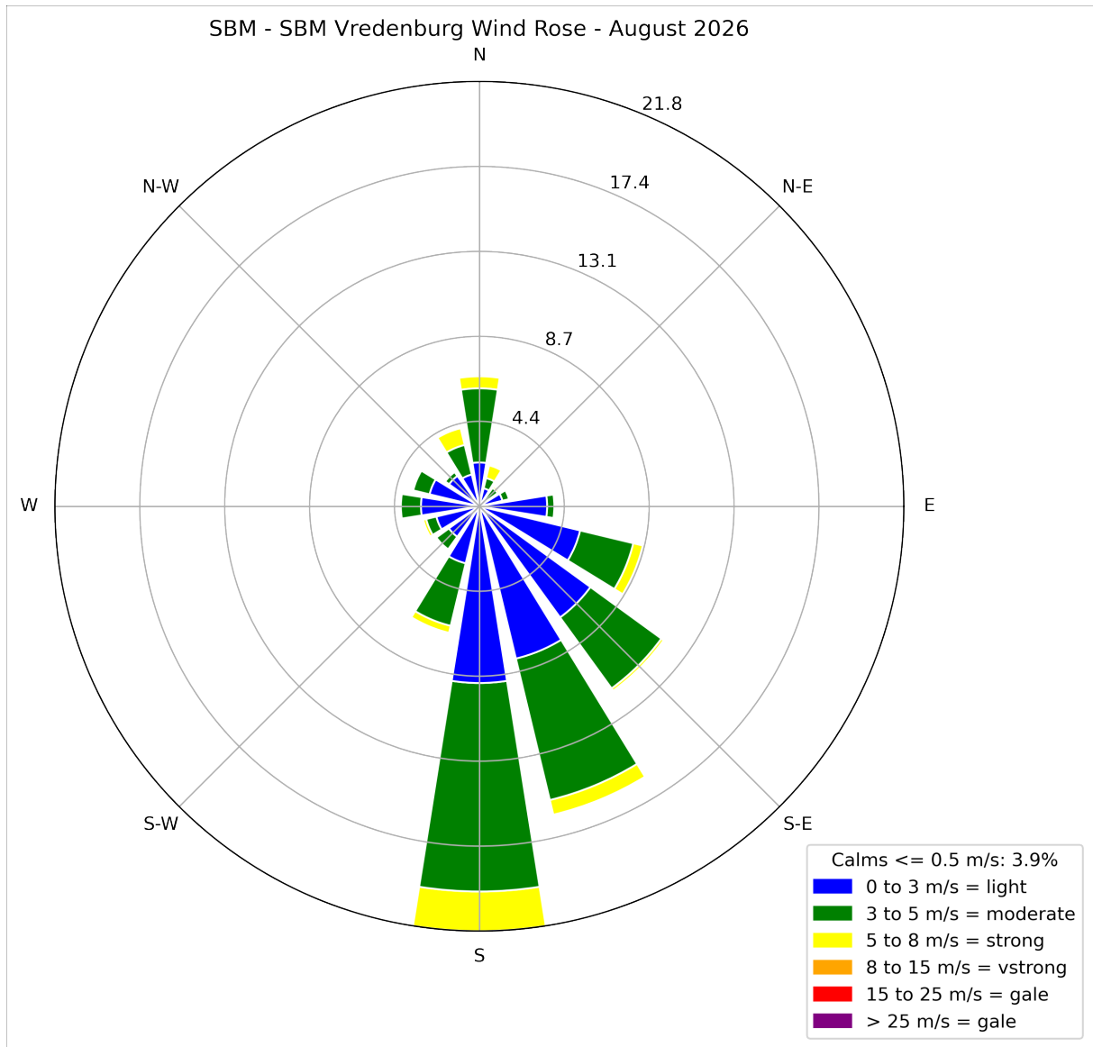
Figure 4.6-2 Wind Rose for Vredenburg for August 2026
